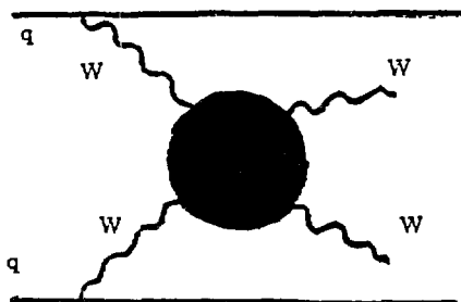
Figure 1: Production of W pairs by WW fusion.
