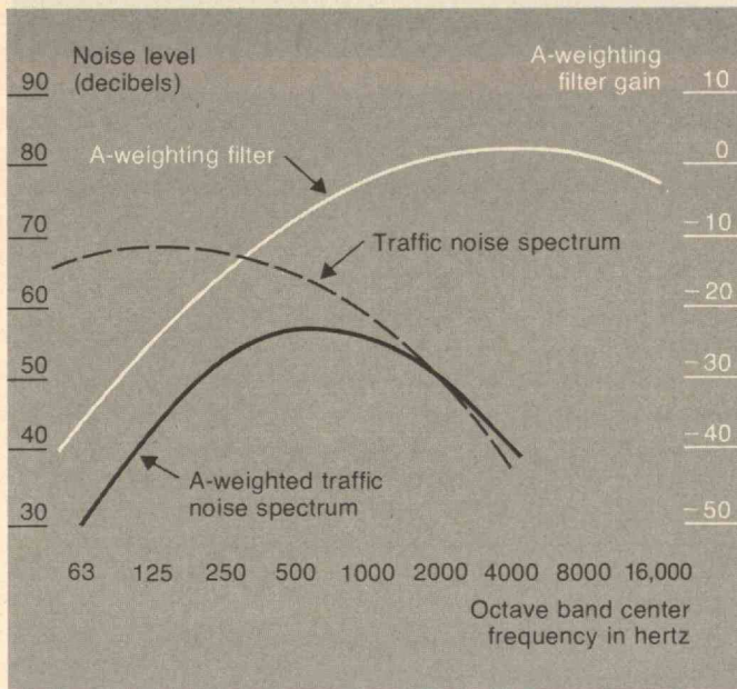
The diagram at the left shows the acoustical modeling system developed for the National Science Foundation, to be used by architects and engineers in designing building projects for lowest noise levels. The filter performs so-called "A-weighting," giving more emphasis to more noisome higher frequencies. The results of this filtering on urban noise is shown in the graph above.
