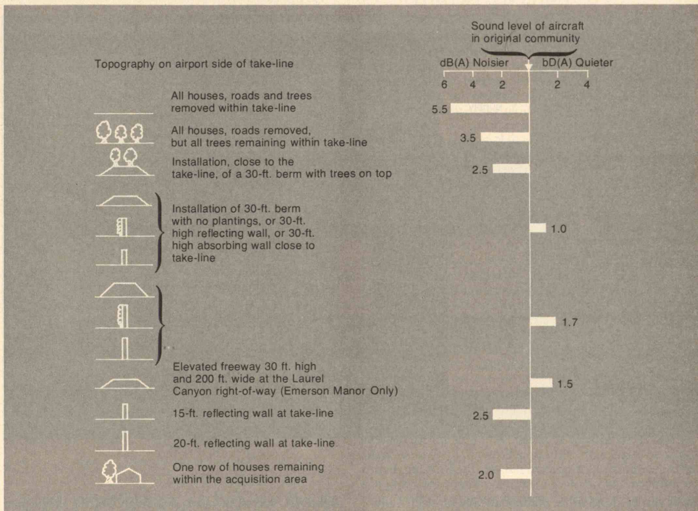
The attenuation of sound by barriers at an airport take-off line. Results of the author's studies of Los Angeles Airport.
